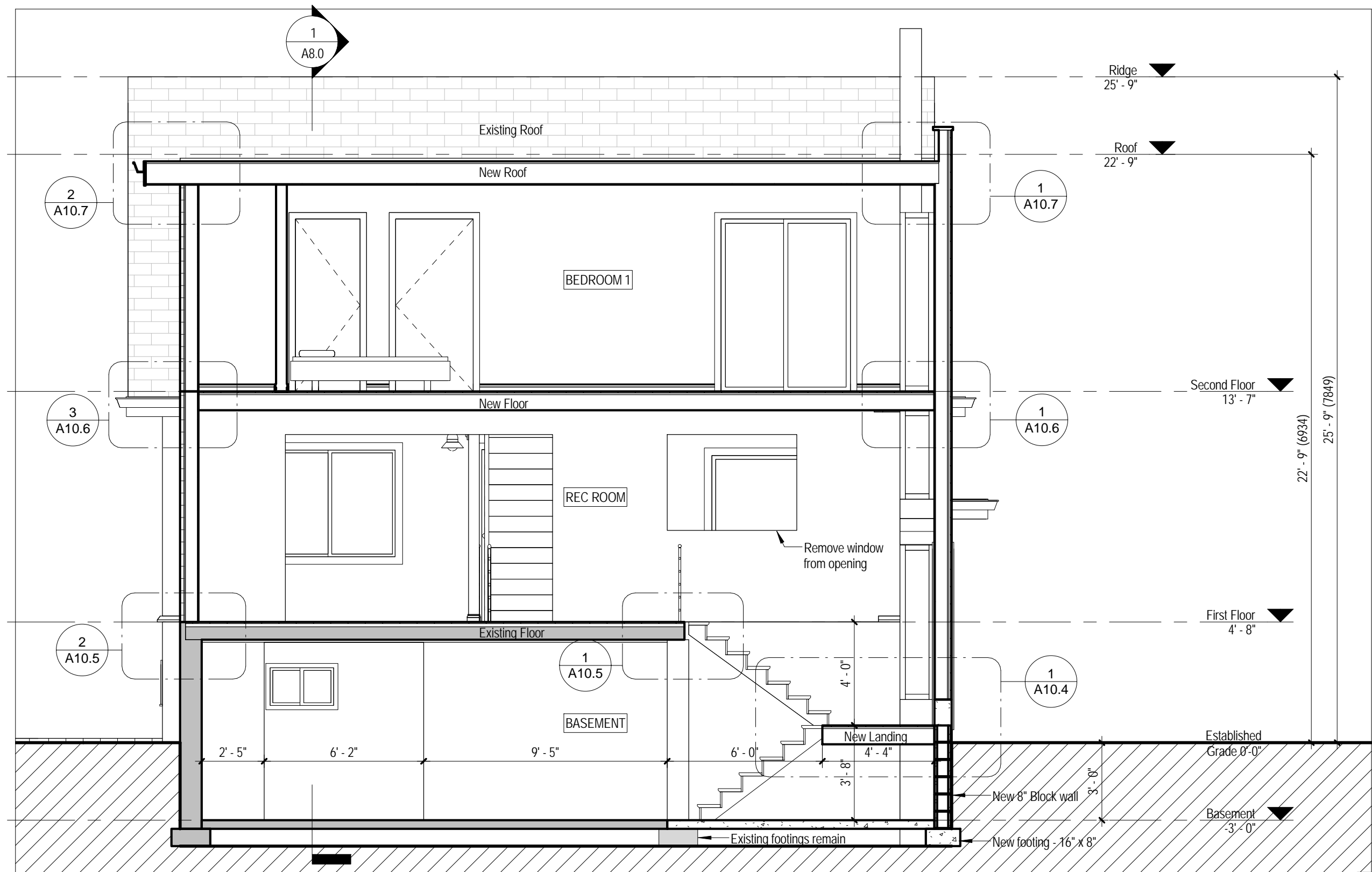
1 Section B 1/4" = 1'-0"
