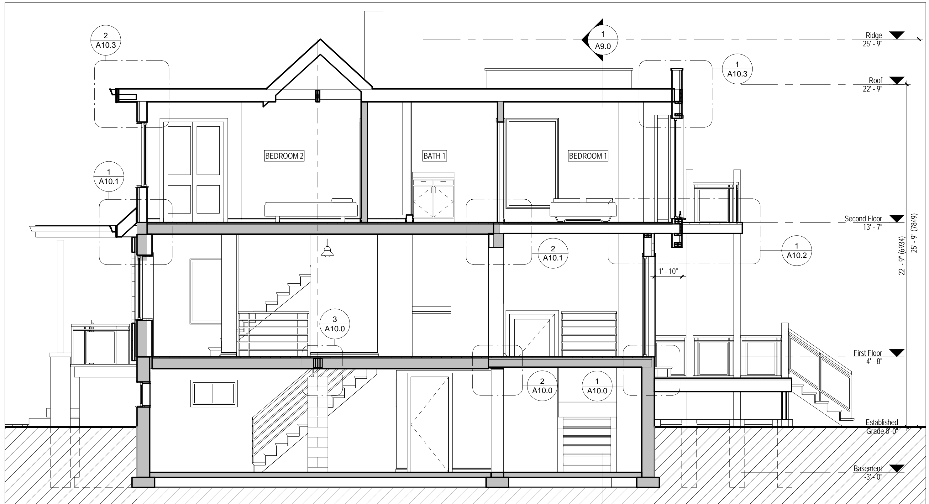
2 Partial Section 1/4" = 1'-0"
