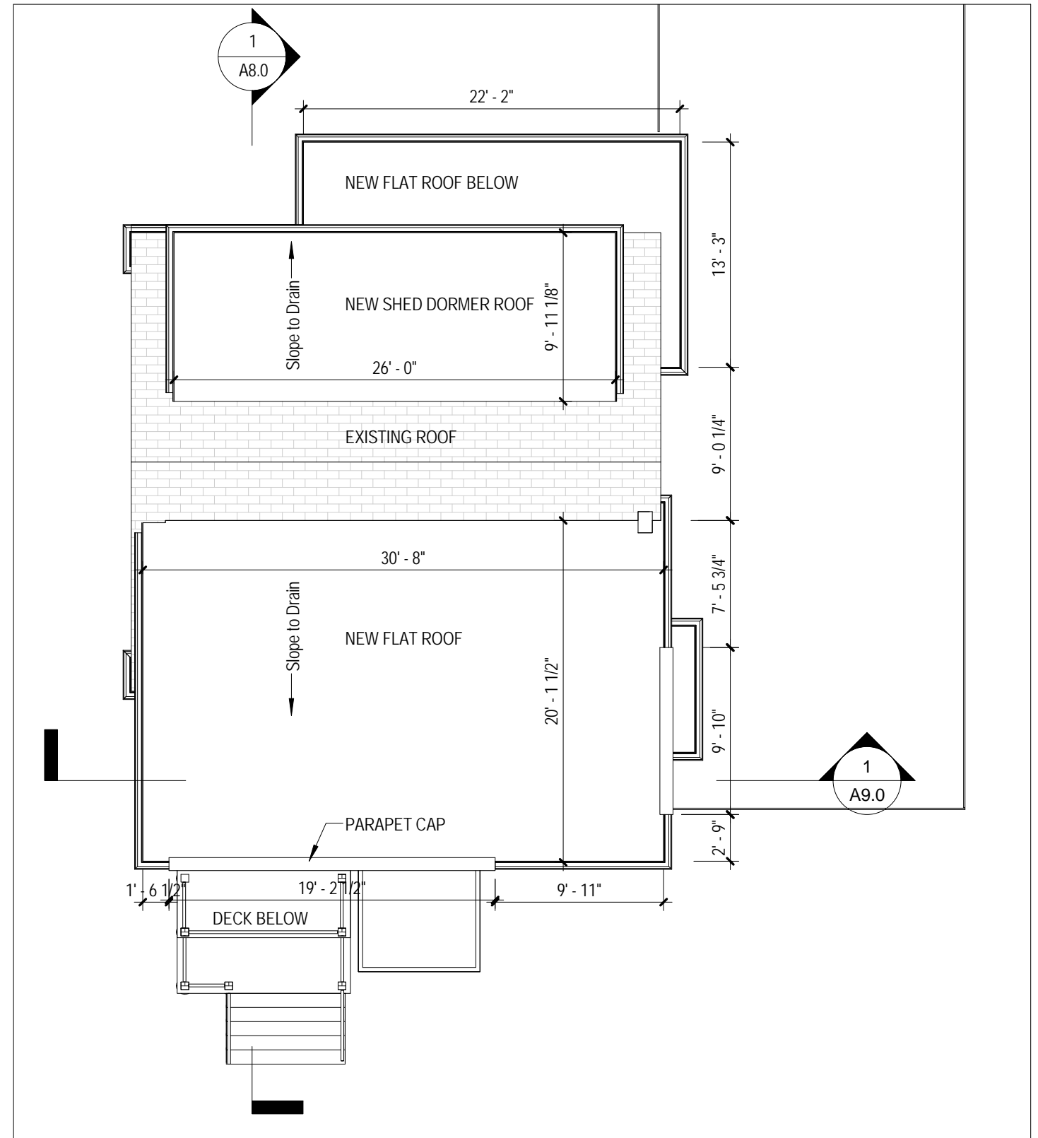
1 Roof Plan 1/8" = 1'-0"
