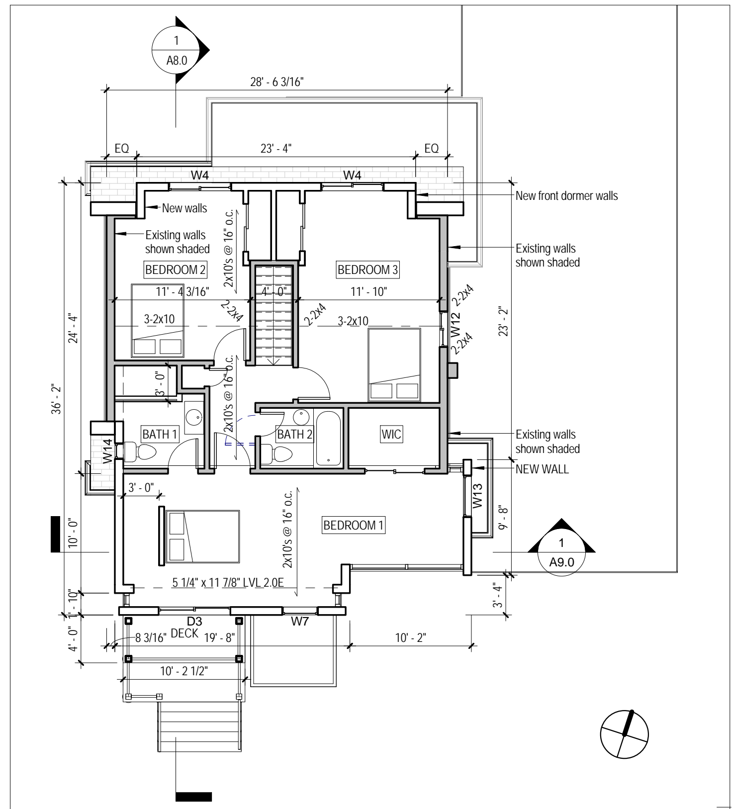
1 Second Floor 1/8" = 1'-0"
