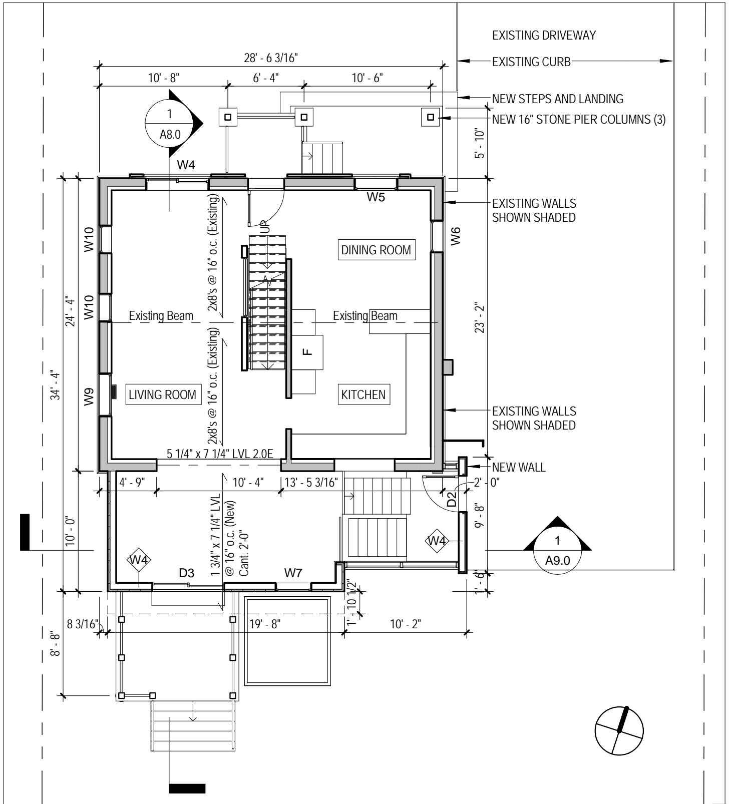
1 First Floor 1/8" = 1'-0"
