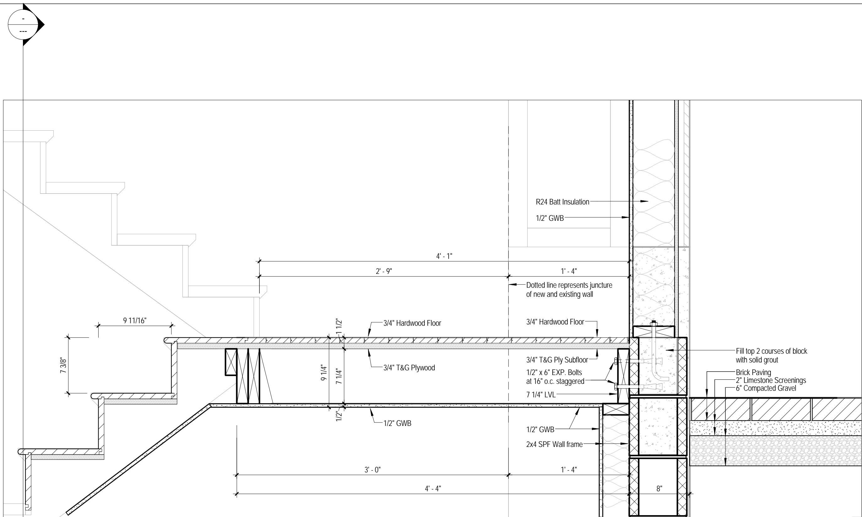
1 Section at Stair Landing 1 1/2" = 1'-0"
