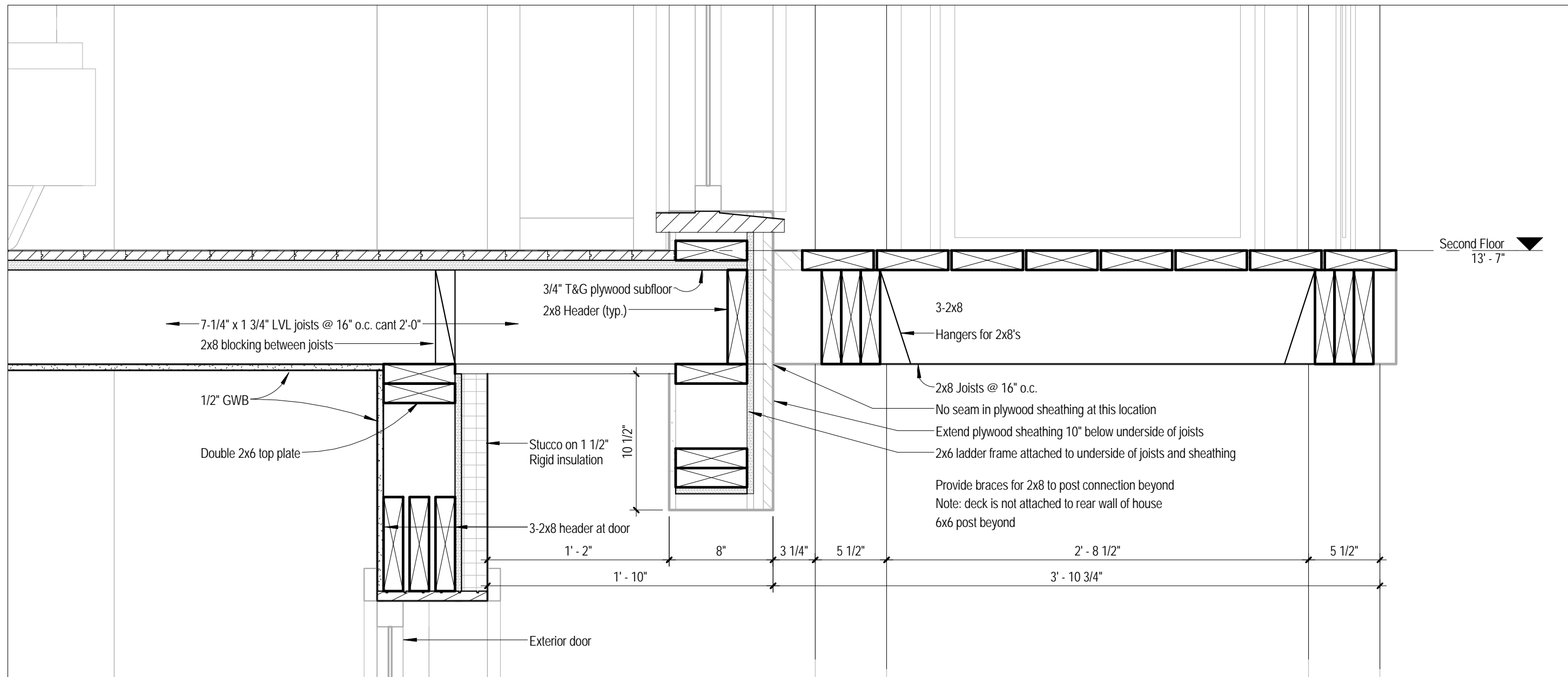
1 Section at Rear Wall and Floor 1 1/2" = 1'-0"
